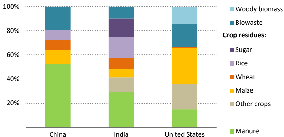
Figure 3.3 ► Feedstock potentials in China, India and the United States
