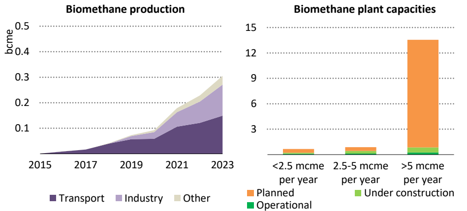
Figure 1.10 ► Biomethane production by use, 2015-2023, and status of plant capacities in 2025, in India
